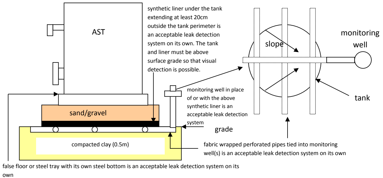
Figure 1. Aboveground Storage Tank Clay Liner Leak Detection System
