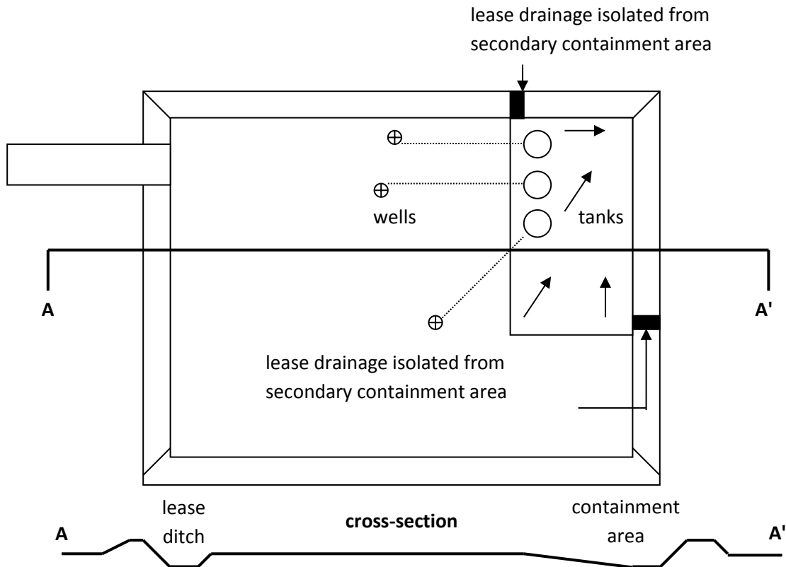
Figure 2. Example Sketch of a Contoured Lease
