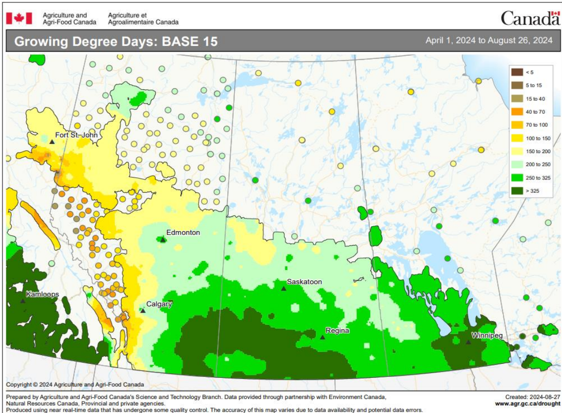
Figure 1: Growing degree days for the prairie provinces, Base 15°C (August 26, 2024) 2
