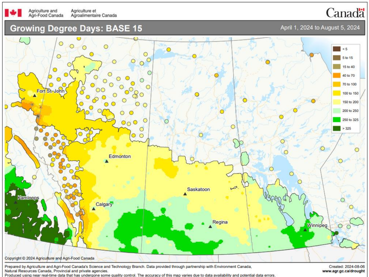
Figure 1: Growing degree days for the prairie provinces, Base 15°C (August 05, 2024) 2
