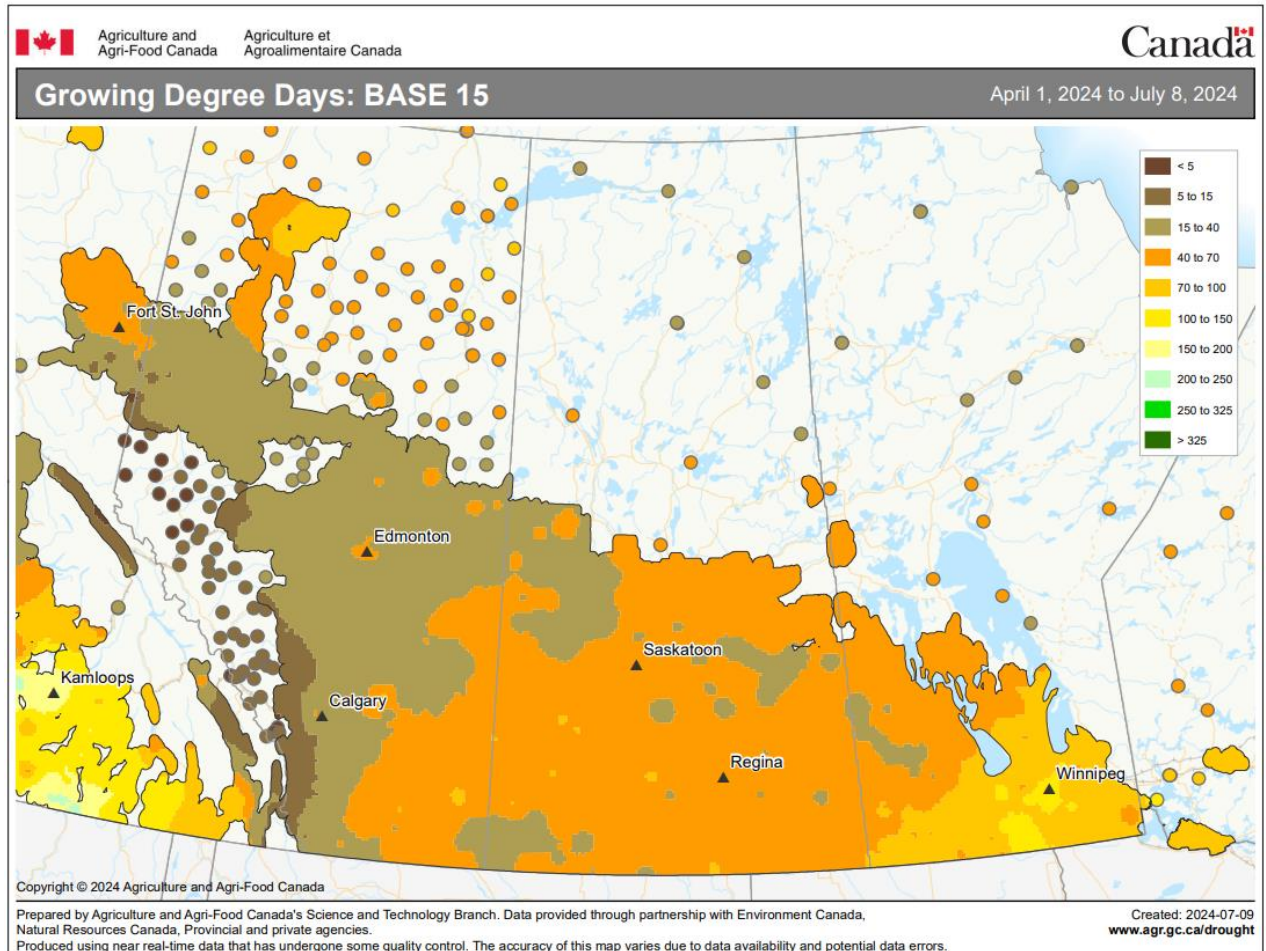
Figure 1: Growing degree days for the prairie provinces, Base 15°C (July 08, 2024) 2
