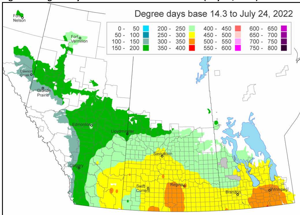
Figure 1: Degree day accumulation Prairie Provinces (July 24, 2022)
