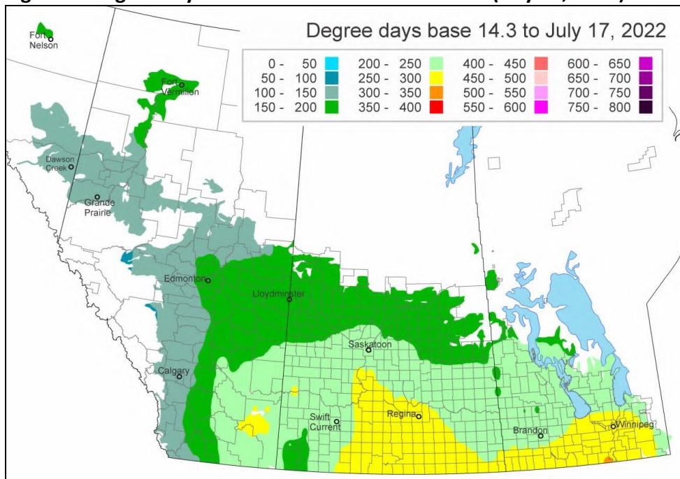
Figure 1: Degree day accumulation Prairie Provinces (July 17, 2022)
