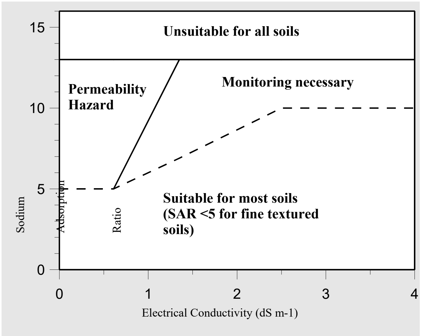
Figure 1: Recommended guidelines for use of sodic waters in irrigation applicable to 95 per cent of the soils in Saskatchewan (Steppuhn and Curtin, 1993).
