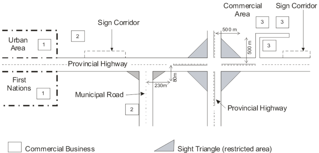
Figure 1220-1 Allowable Private Signing
